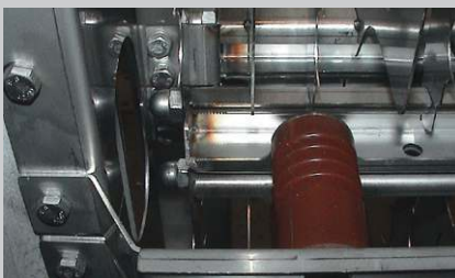
Removable PSP-Ionizer
